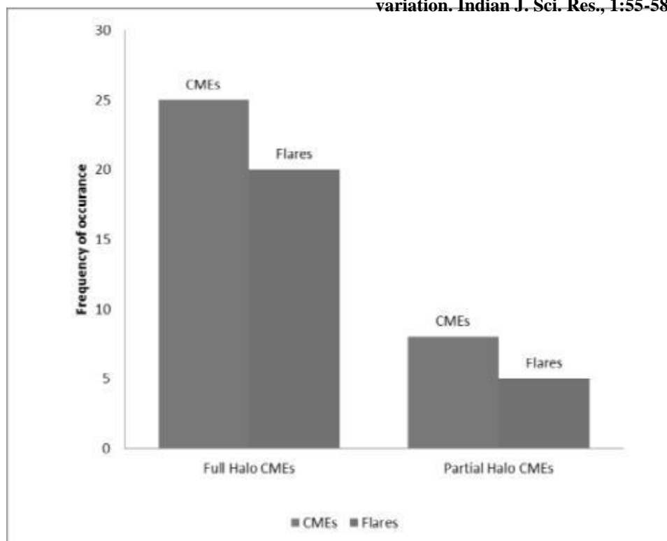
Fig. 2: Association of Full Halo CMEs and Partial Halo CMEs with flares on Cosmic ray decrease variation. Indian J. Sci. Res., 1:55-58.
