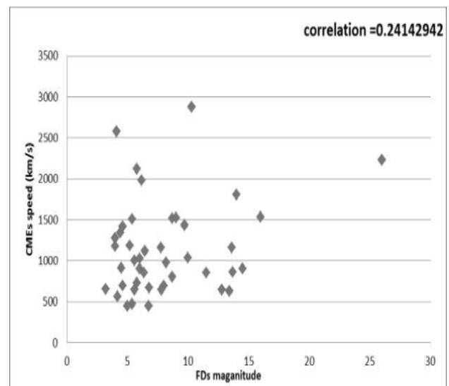
Fig. 1: Association of FDs magnitude with CMEs speed
